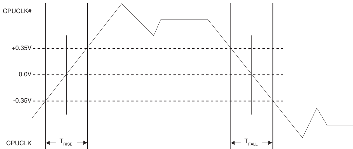
Figure 2 - 0.7V Differential TRise and TFall Measurement Points
